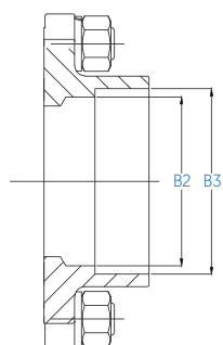
Socket Weld End
