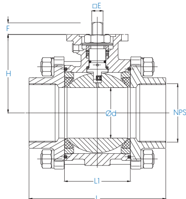
NPS 2" - 3" Fire Safe - NPS 2"
